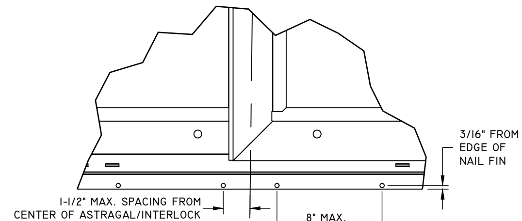
DETAIL B - ALTERNATE 2-TRACK SILL ONLY
