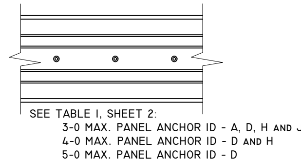
INTERLOCK / ASTRAGAL PATTERN
