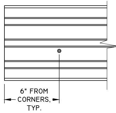
END HOLES
